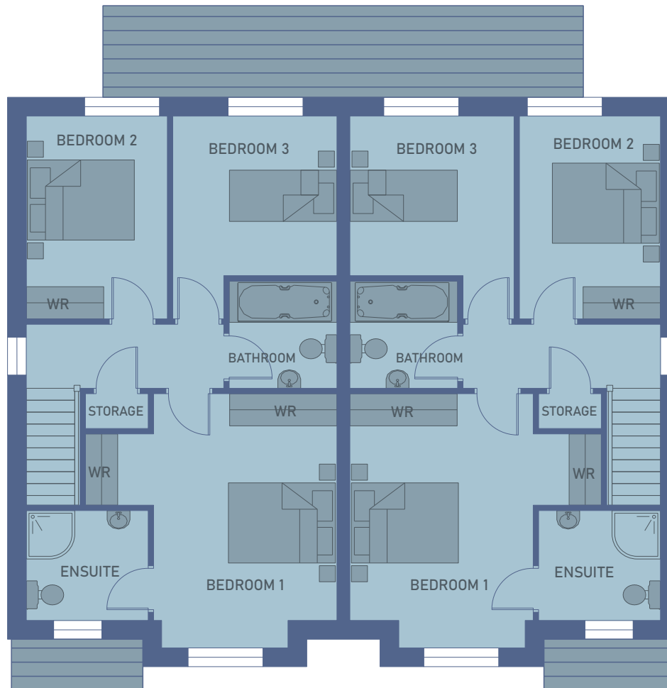
3 BEDROOM UNIT - FIRST FLOOR 55.62 SQMT
